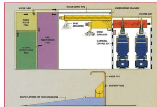
ABOVE: Diagram of concrete reclaimer set-up.
